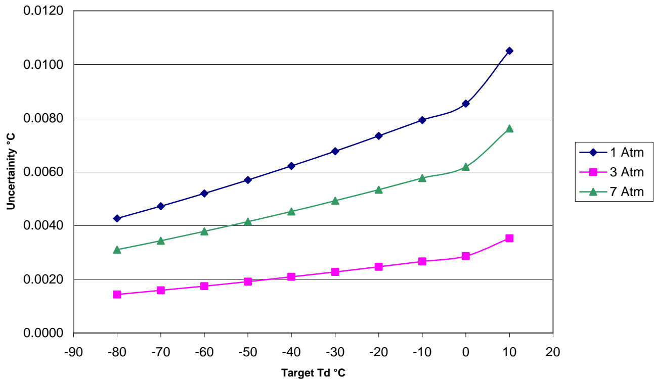
Figure 3. Uncertainty contribution at 1, 3 & 7 atmospheres.
